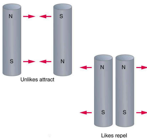
Figure 22.5 Unlike poles attract, whereas like poles repel.
